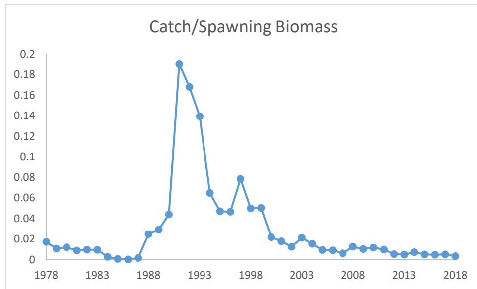
Figure 1. Catch:female spawning biomass ratio using spawning biomass for Dover sole only.
