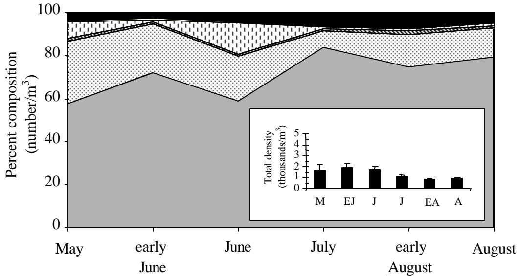
Figure 3.—Monthly zooplankton composition (percent number per m 3 ) and total density (thousands per m 3 ) in shallow (20-m) and deep (=200 m), 333- \mu\text{m} mesh, bongo net samples from Icy Strait in the northern region of southeastern Alaska, May–August 2003. Total density means and standard errors are based on four samples in each time period. NS = no sample.
